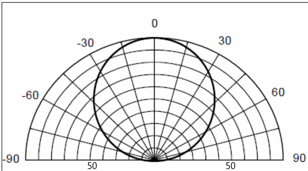
Directivity
